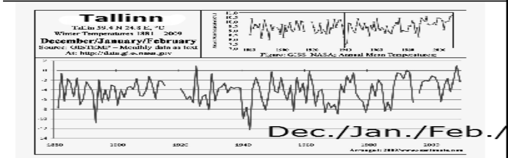
Abb. E3-7; Winter-T°C, Dez/Jan/Feb, 1880-2010
